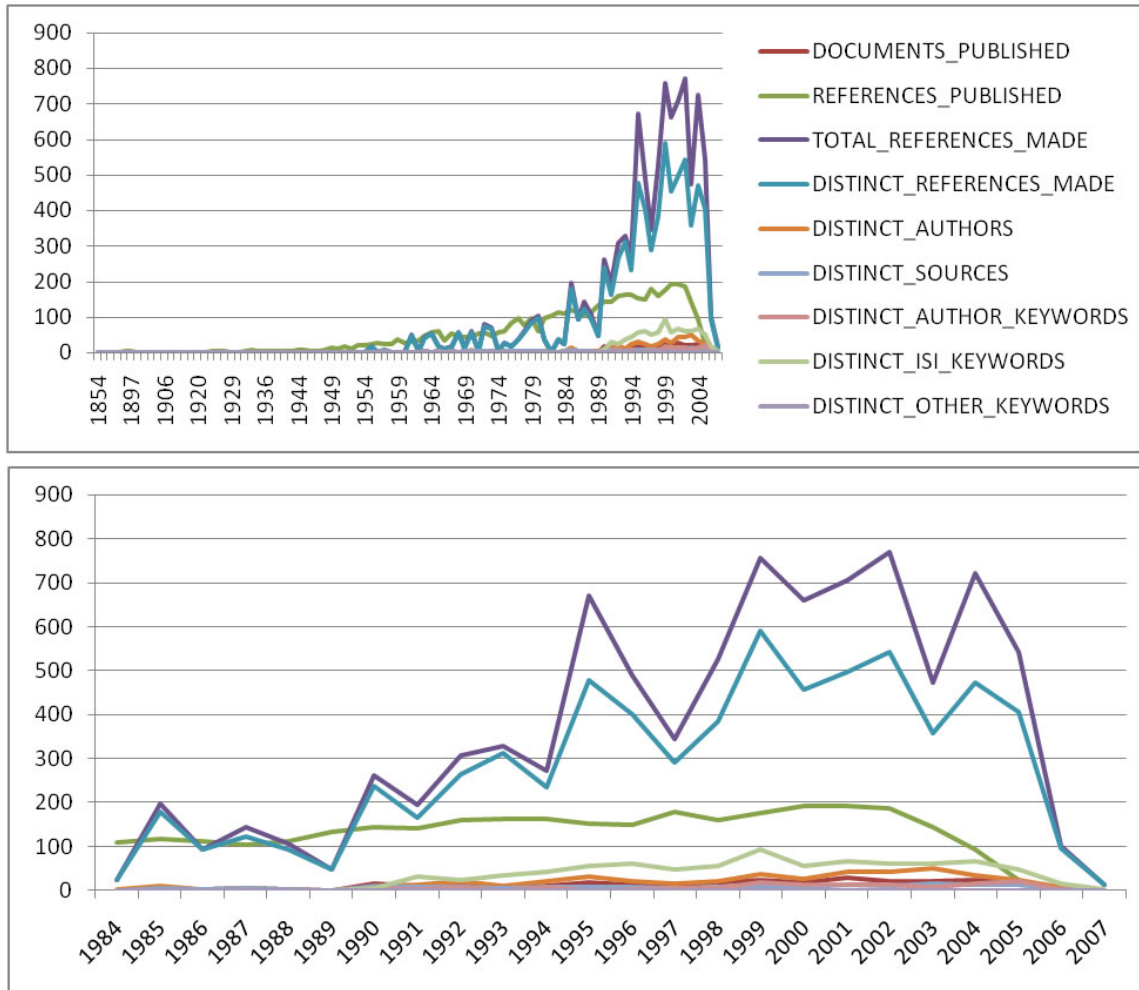
Figure 5.20: Longitudinal study of 'FourNetSciResearchers'
