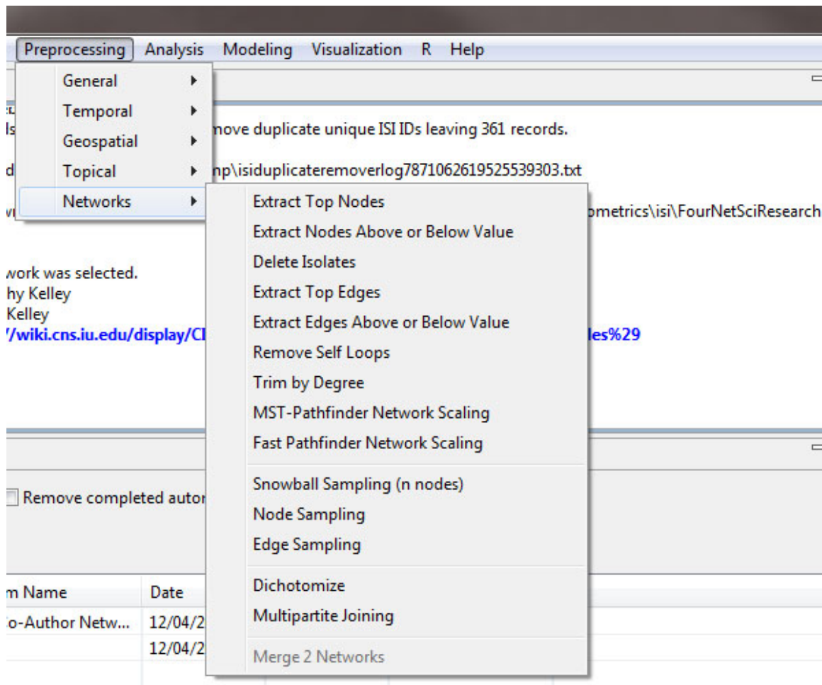
Figure 2.8: Preprocessing options
