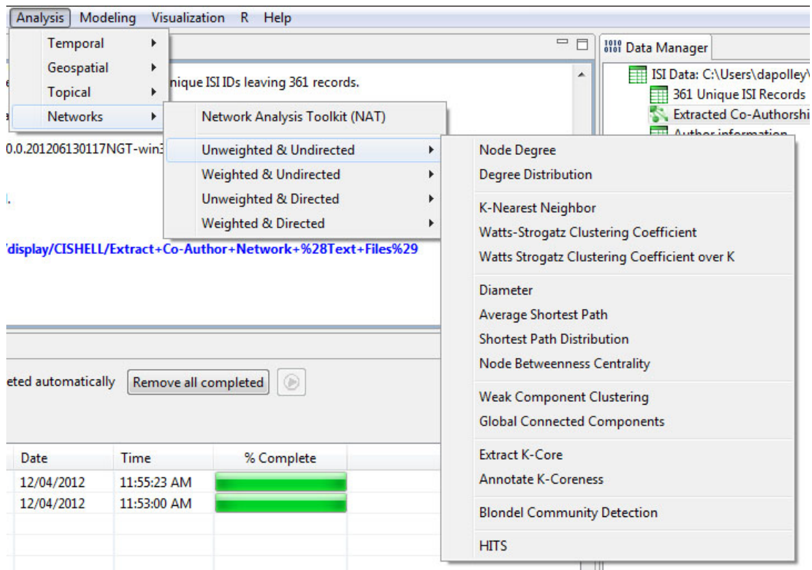
Figure 2.9: Analysis options
