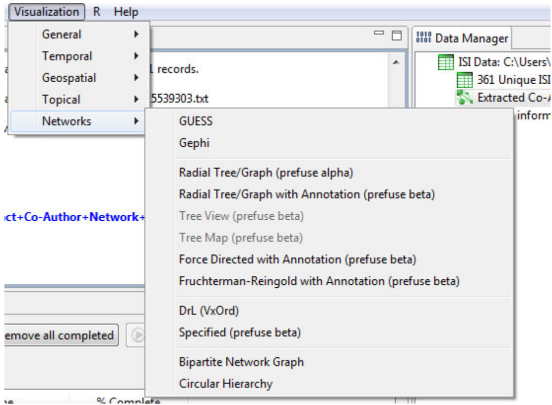
Figure 2.11: Visualization options
