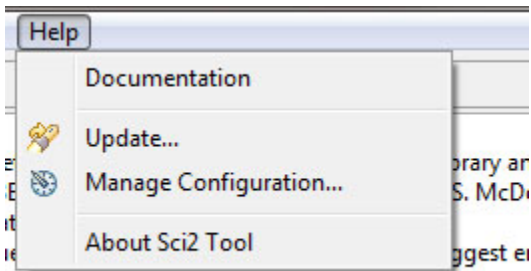
Figure 2.13: Help options
